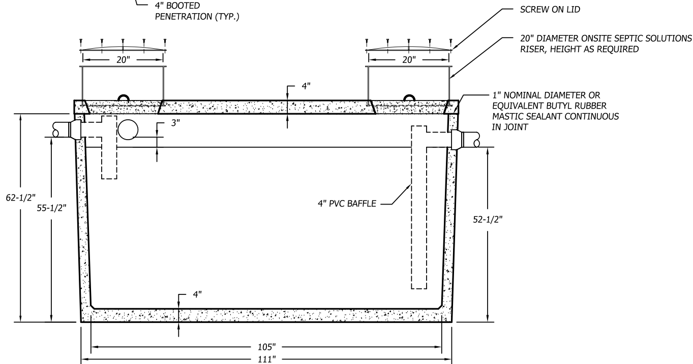
SECTION
